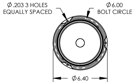
FLANGE or PIPE MOUNT - PIPE SIZE - 1-11 1 / 2 NPT
